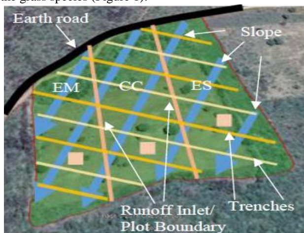
Figure 1. General layout of project site and grass plots distance
